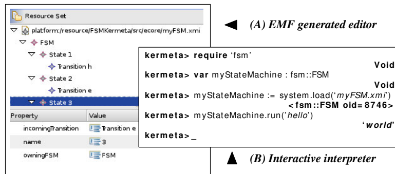
Fig. 13. KerMeta editor and interpreter
