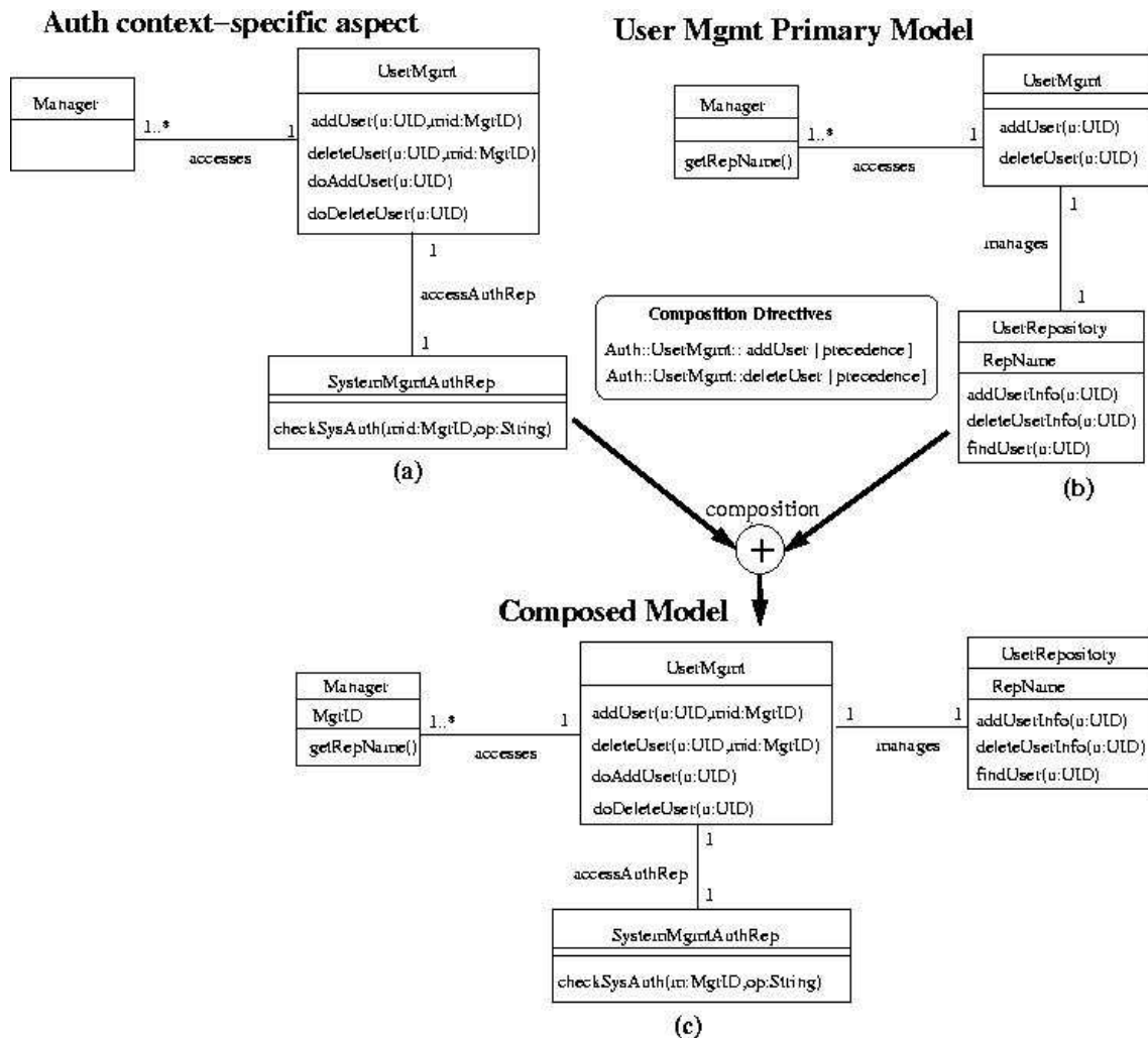
Figure 3 - A simple model composition example
