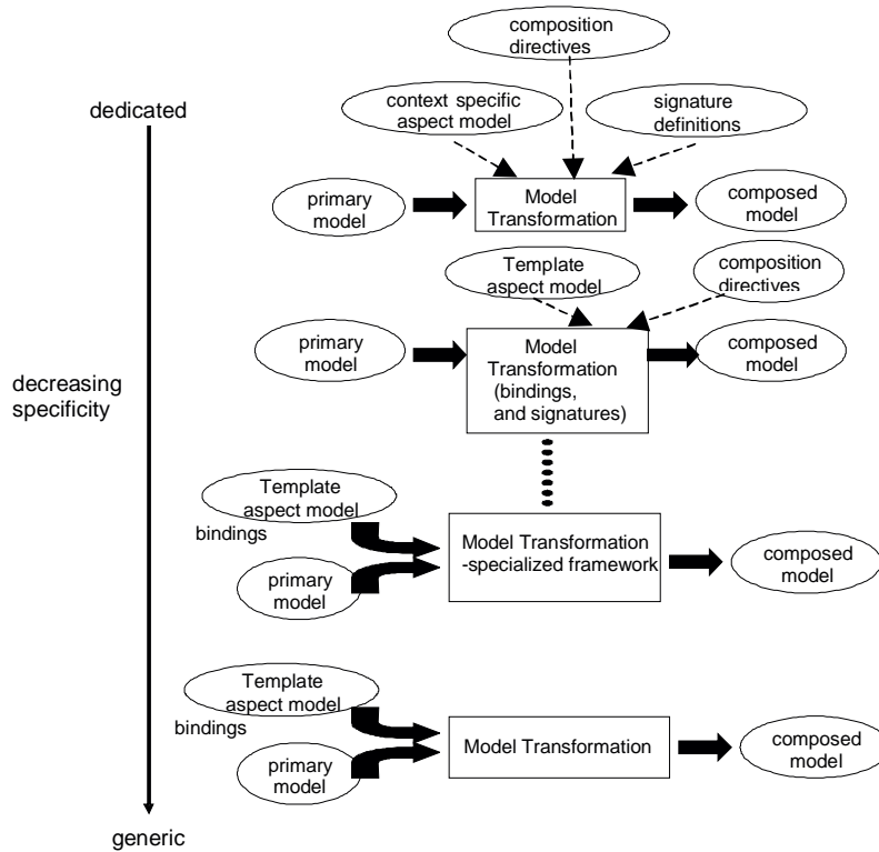
Figure 2 - Intermediate variants from dedicated to generic composition
