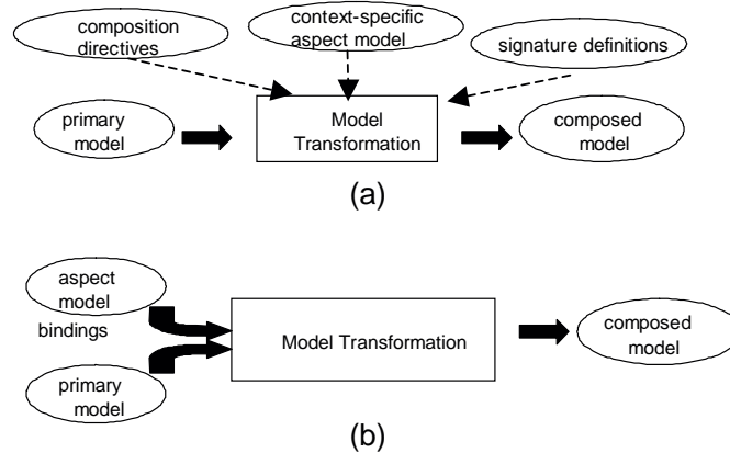
Figure 1 - two transformation-oriented composition approaches
